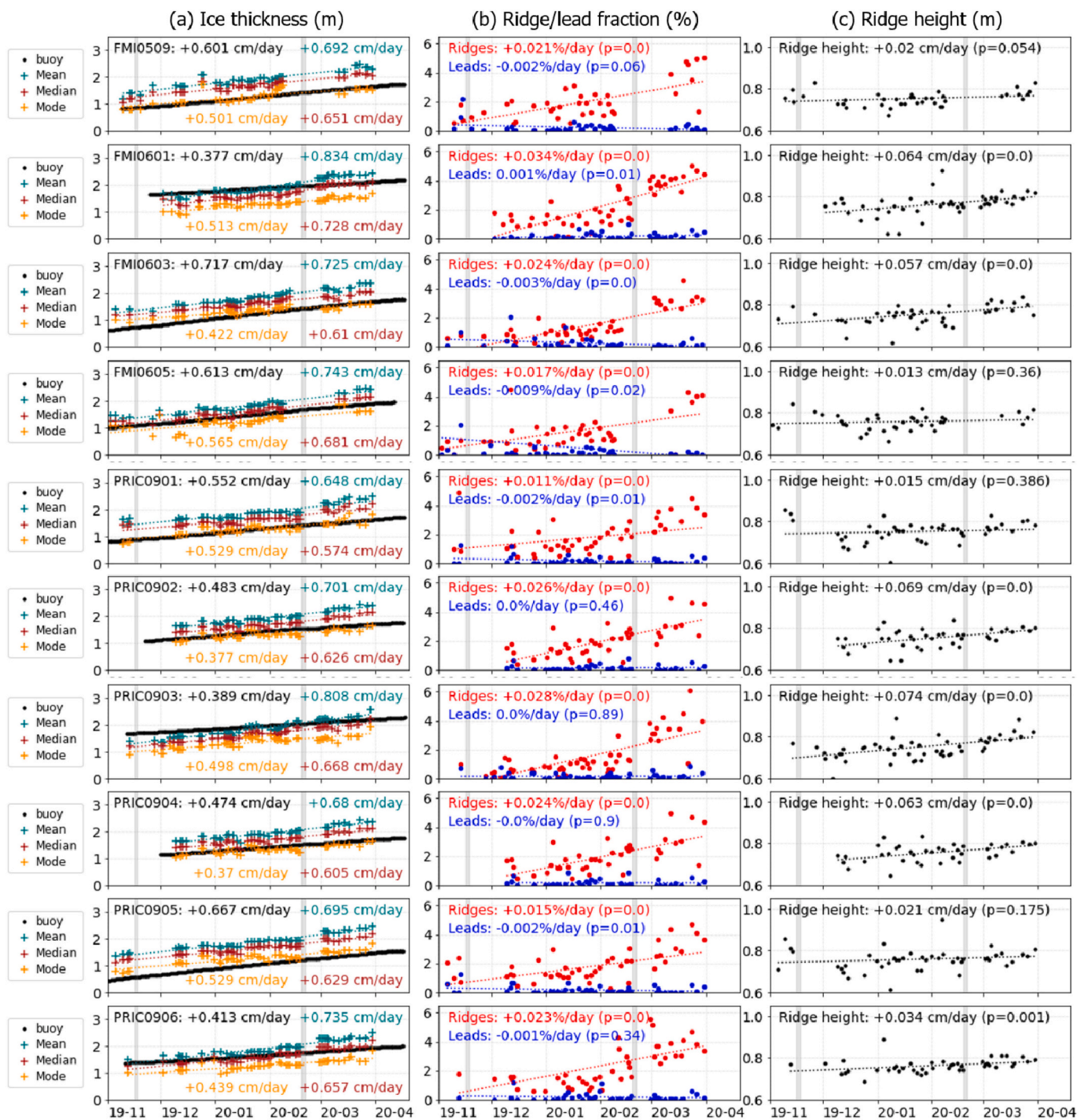
Fig. 8. (a) Temporal variations of buoy ice thickness (black line), nearby IS2 modal thickness (orange crosses), IS2 median thickness (brown crosses), and IS2 mean thickness (green crosses) for 10 SIMBA buoys; (b) temporal variations of ridge fractions (red dots) and lead fractions (blue dots) estimated by the IS2 data within 20 km from each buoy; (c) temporal variations of ridge heights estimated by the IS2 data within 20 km from each buoy. Gray shading vertical bars indicate the heavy storm events with dramatic increases in wind speed in mid-November and mid-February. (For interpretation of the references to colour in this figure legend, the reader is referred to the web version of this article.)
